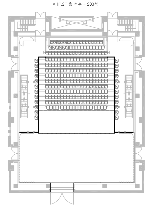
ARENA STAGE
