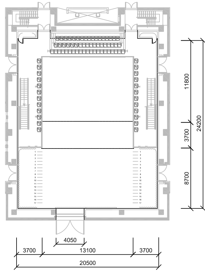
THRUST STAGE
